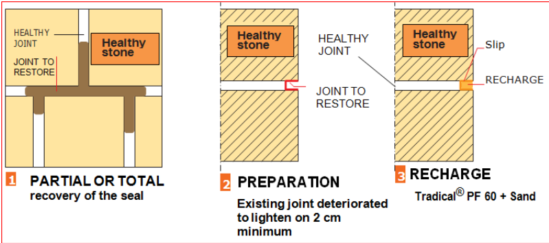
Fig. 7. Repair of the facings and pointing
